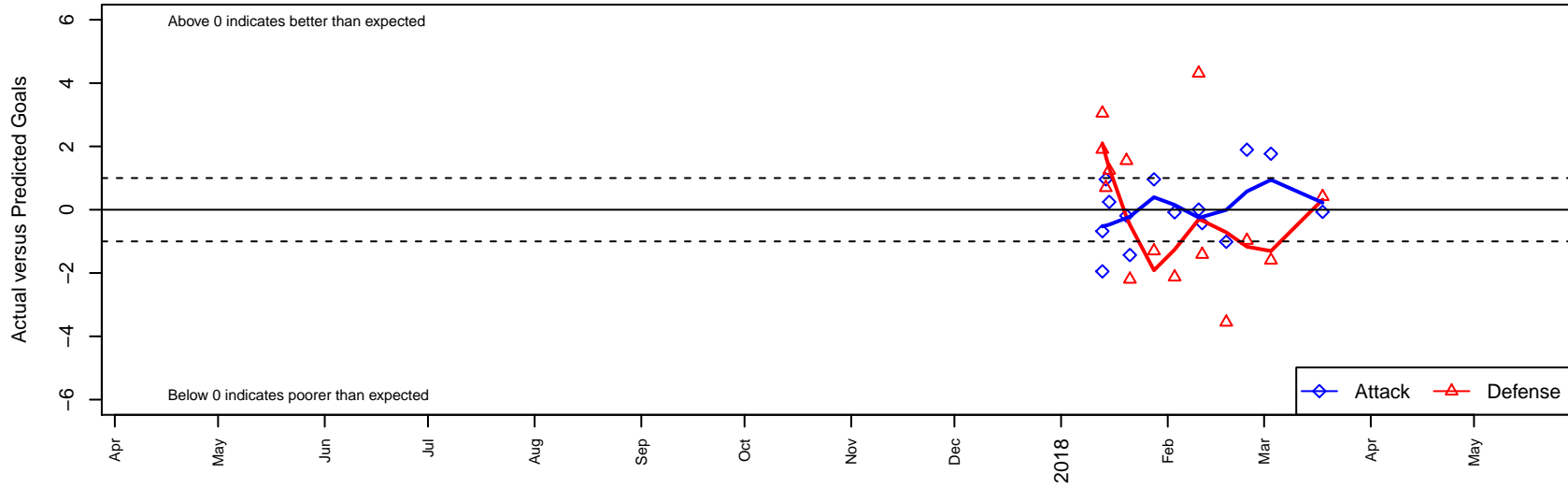
GPS Oregon B99 Dots are actual minus expected GF (blue circles) and GA (red triangles). Blue line is smoothed change in attack strength. Red is smoothed change in defense strength.
